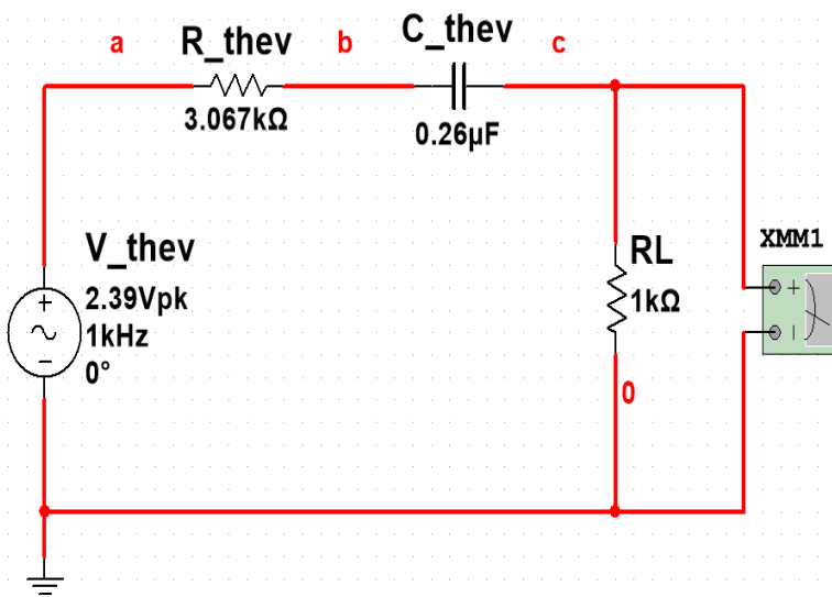
Fig.B.2: Thevenin's Equivalent circuit
